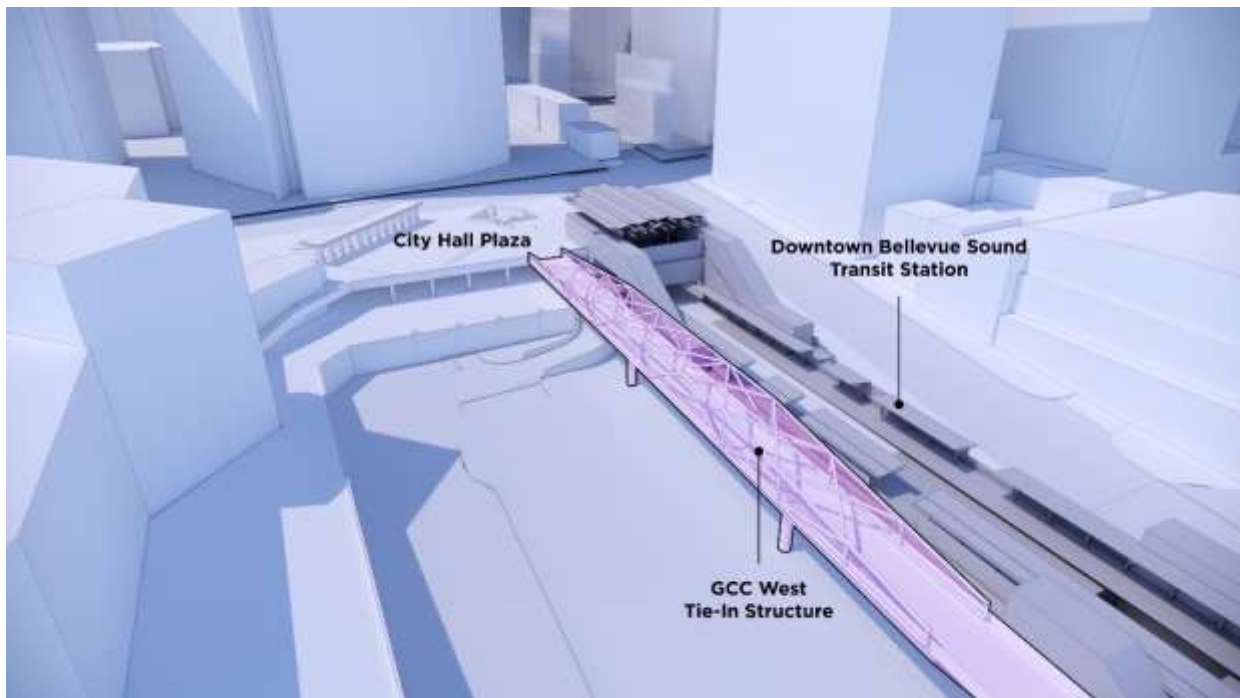
Figure 44: Conceptual rendering of west tie-in structure, Steel Truss Cantilever.
