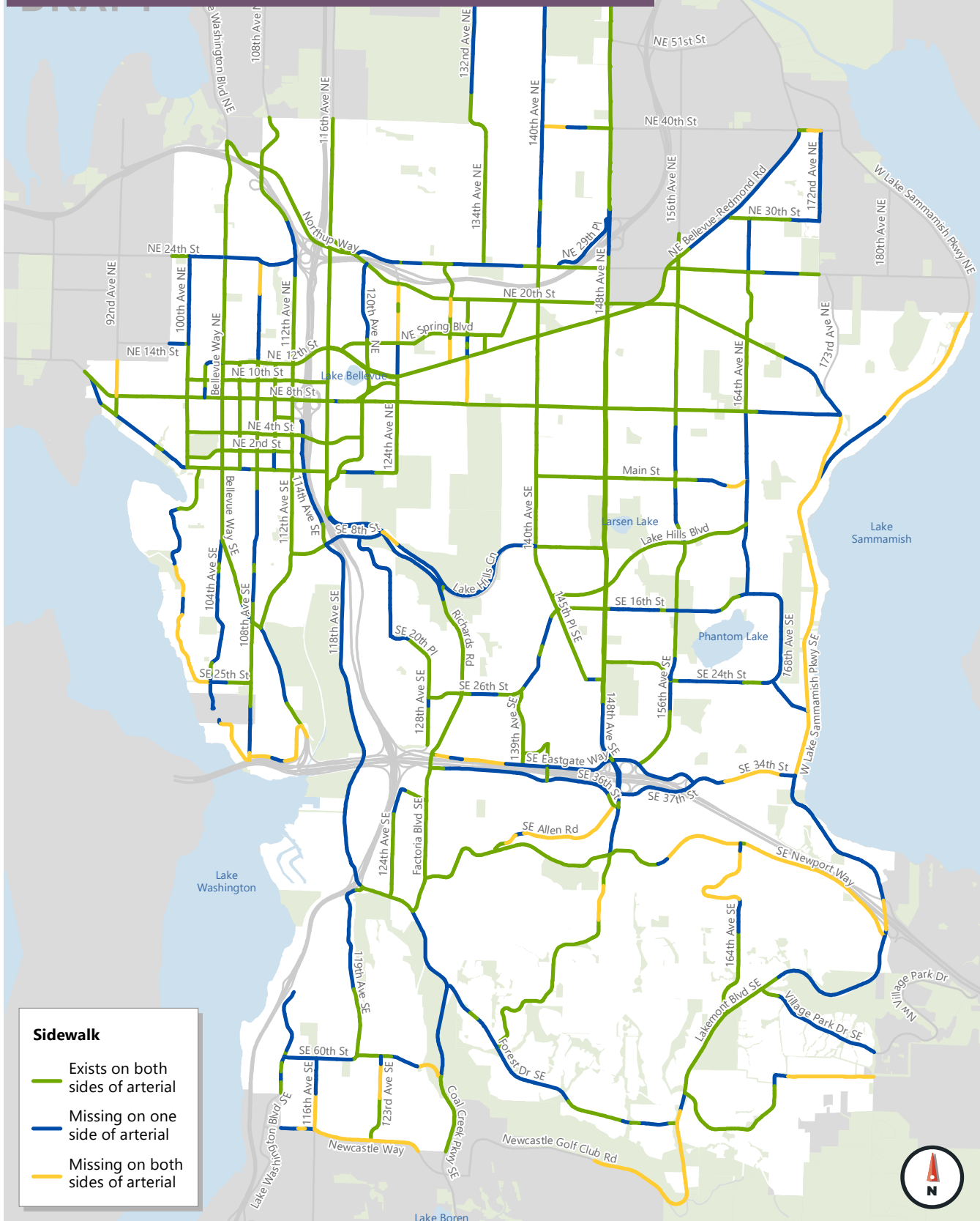
Figure 14: Pedestrian Network Performance – 2021
